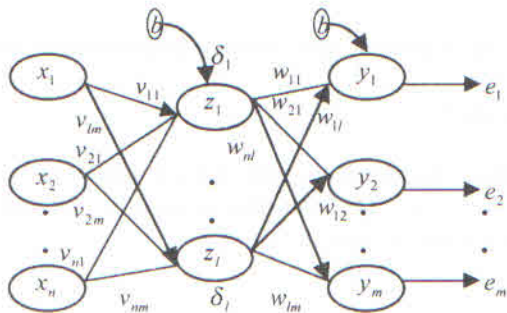
FIGURE 4. The BP architecture
