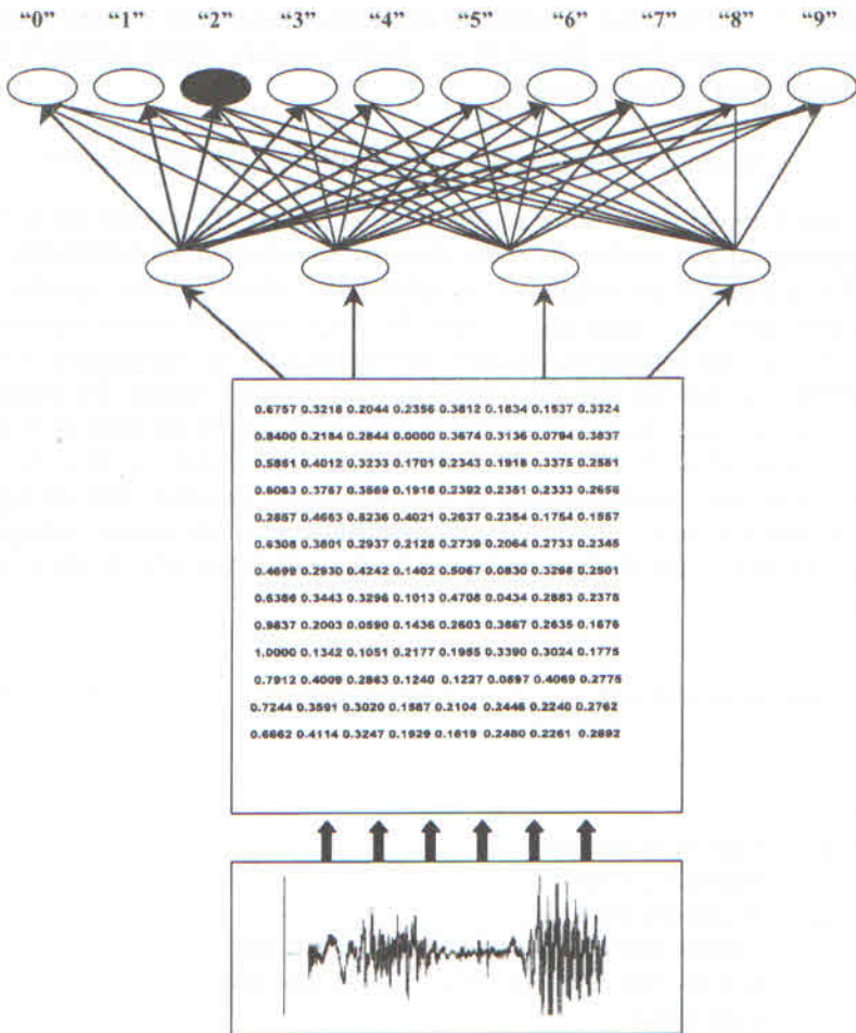
FIGURE 3. The process of recognition for utterance "2"
