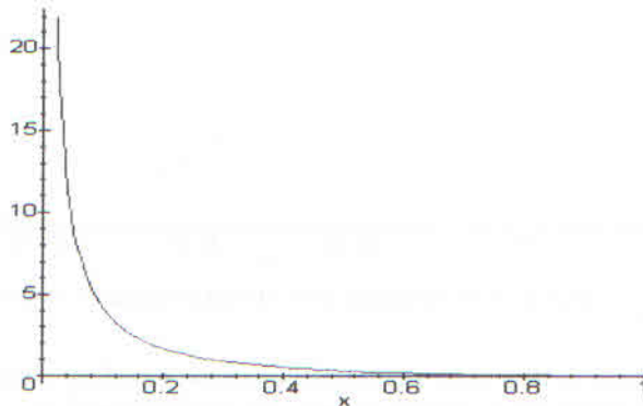
FIGURE 6. Proposed error function of backpropagation model
